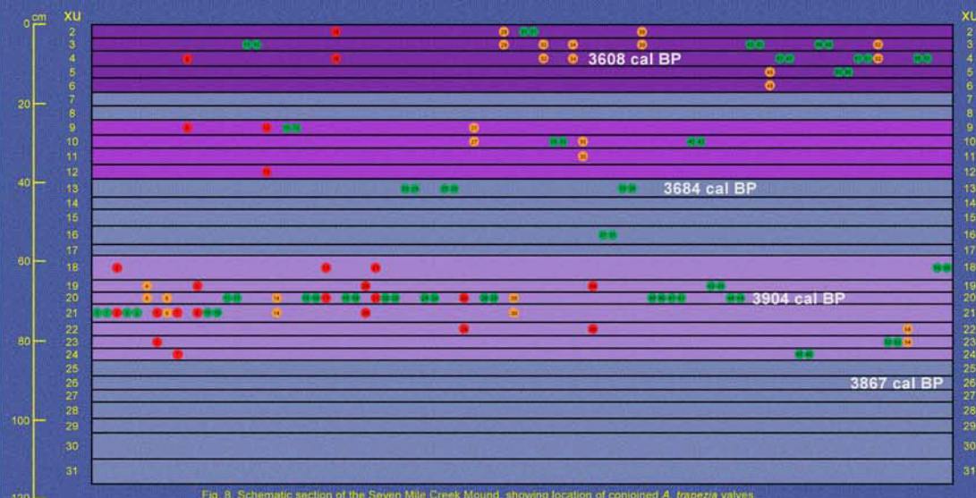
Fig. 8. Schematic section of the Seven Mile Creek Mound, showing location of conjoined A. trapezia valves.
